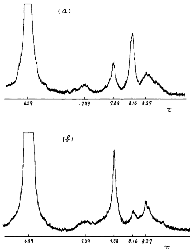
Fig. 1.—N.m.r. spectra of methyl acrylate- \alpha,\beta\text{-}d_2 polymers prepared with (a) azobisisobutyronitrile in toluene at 50^\circ and (b) lithium aluminum hydride in toluene at -78^\circ . The spectra are measured on 10% solutions of the polymers in benzene.
